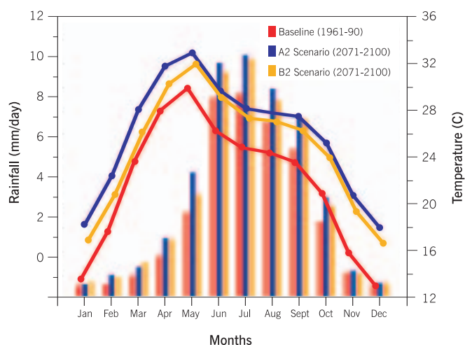
Figure 2.2 Mean Annual Cycles of All-India Rainfall and Temperature, Baseline and Simulated
