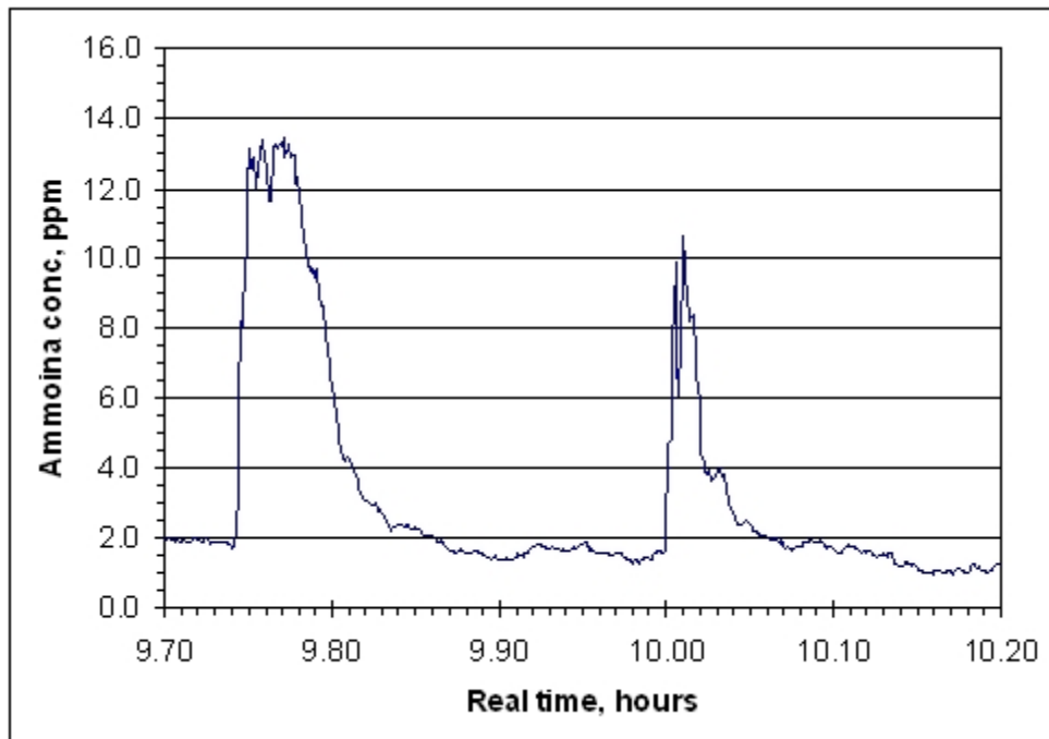
Figure 5: example of a record of measured concentration of ammonia in response to two injections of ammonia from a gas cylinder.
