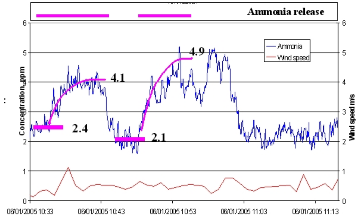
Figure 4: example graph of ammonia emission in response to two controlled releases of ammonia from a controlled source. Back ground emission is indicated in each case as well as the perceived steady state concentration following a period of release.
