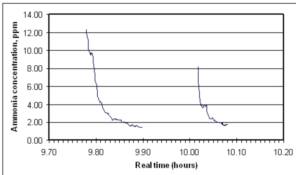
Figure 6: decay curves from previous example.
