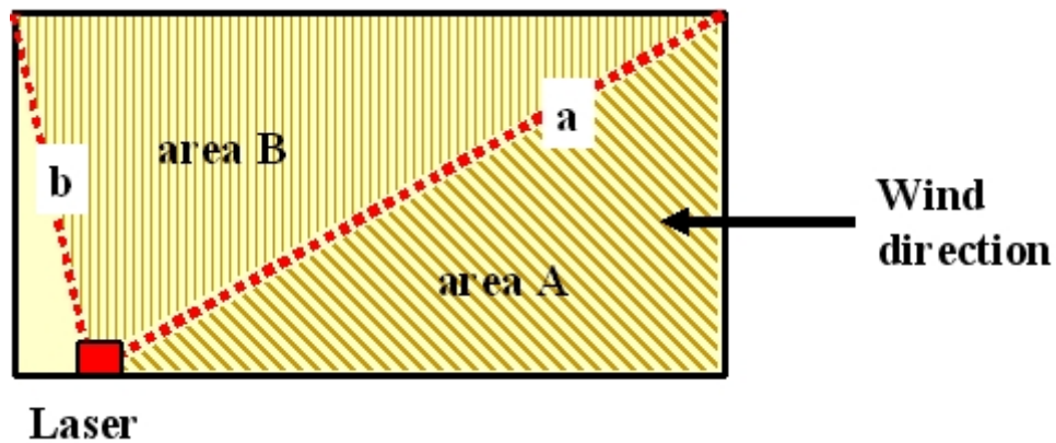
Figure 3: geometry of laser location with respect to the building being monitored.
