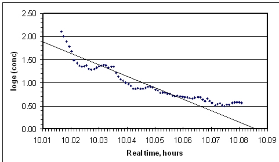
Figure 8: plot of \log_e C against time, t for the second curve in Figure 6.
