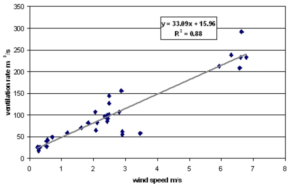
Figure 10: ventilation rate as a function of wind speed for a given building.
