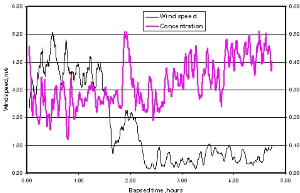
Figure 9: wind speed plotted against ammonia concentration in the livestock building.
