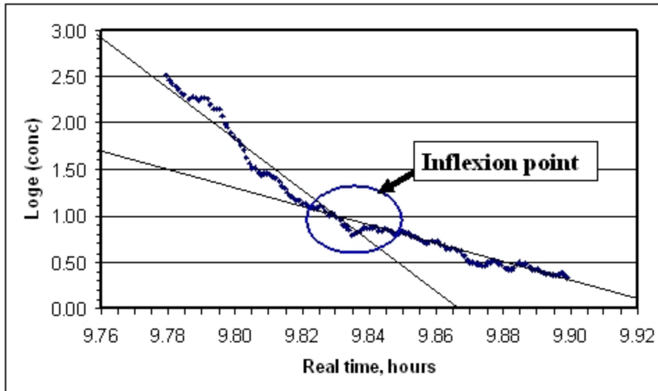
Figure 7: plot of \log_e C against time, t for first curve shown in Figure 6.
