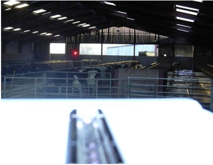
Figure 2: laser equipment (foreground) set up to send a beam across a farm building. The mirror reflecting the beam is just distinguishable in the distance.
