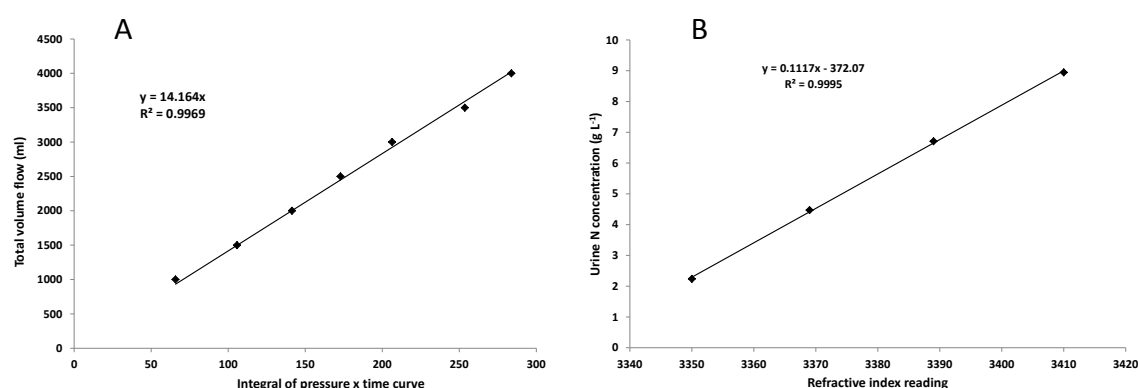
Figure 3. Urine volume (A) and N concentration (B) calibration curves for one of the urine sensors used in the study
